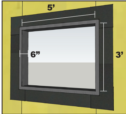
VAPROLIQUI-FLASH : 1 Sausage Flashing: REVEALFLASHING MECHANICALLY ATTACHED Rough Opening = 5' x 3' x 6"
