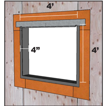
VAPROLIQUI-FLASH : 1 Sausage Flashing: VAPROFLASHING MECHANICALLY ATTACHED Rough Opening = 4' x 4' x 4"
